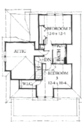
Second Floor Plan 489 square feet
